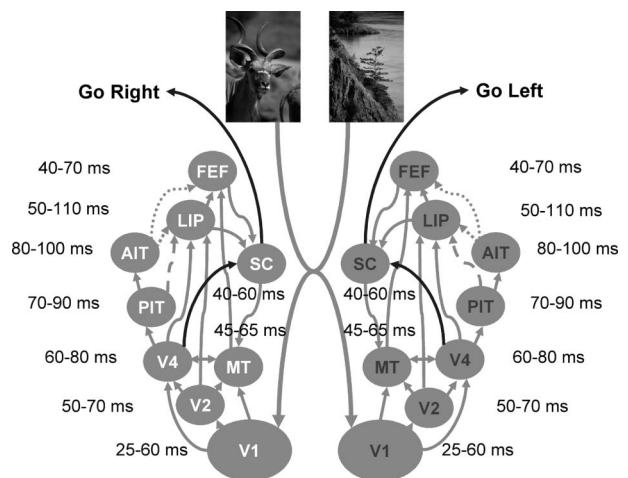
Fig. 9. Flow-chart of anatomical connections between the ventral visual pathway involved in object recognition and the eye fields involved in eye movement control. Latency estimates are based on monkey data, but the corresponding values in humans are probably longer. The first number for each processing stage indicates the approximate latency of the earliest responses of visually responsive neurons to a flashed stimulus, whereas the second number provides a more typical, average latency (Nowak & Bullier, 1997; Thorpe & Fabre-Thorpe, 2001). Arrows from the posterior and anterior inferior temporal cortex are dashed and dotted, because these connections are either insignificant or absent (Bullier et al., 1996; Schall et al., 1995).
