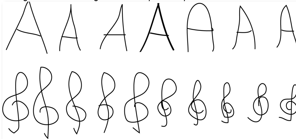
Figure 1.2: The same pattern can look very different...
