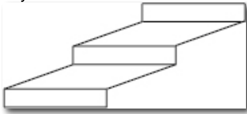
Figure 1.6: A bistable percept. The image can be interpreted in two different ways.
