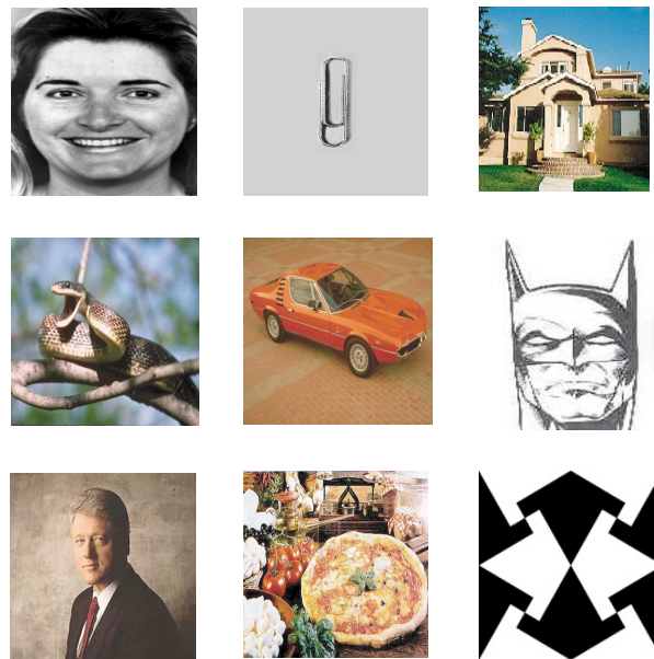
Fig. 2. Sample of stimuli presented in each category. Figures (mostly color) were drawn from a group of nine categories that included faces denoting emotional expressions by unknown actors 21 , household objects, spatial layouts (including house exteriors, interiors and natural scenes), animals, cars, drawings of famous people or cartoon characters, photographs of famous people, food items and abstract patterns. Stimuli were presented for 1000 ms. Subjects had to indicate by pressing a button whether the image was a human face or not.
