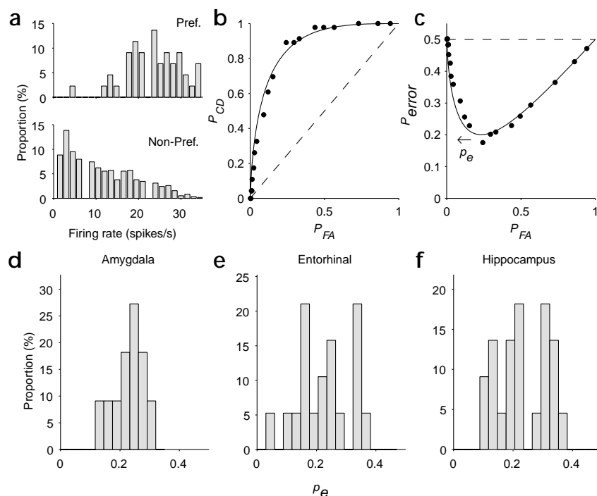
Fig. 6. ROC analysis and p_e distribution. (a) Distribution of firing rates for the neuron shown in Fig. 3 for the preferred category (top, animals) and non-preferred category (bottom, all other categories). Bin size, 1.5 spikes/s. These represent the conditional probability distributions P(f | stim \in preferred\ category) and P(f | stim \notin preferred\ category) , where f denotes the firing response computed in the 100–1000 ms interval and stim indicates the stimulus. (b) ROC analysis. Each stimulus is classified into the preferred category if the firing rate during the 100–1000 ms interval is above a given threshold T . The probability of correctly classifying a stimulus ( P_{CD} ) is plotted as a function of the probability of making a false alarm ( P_{FA} ). This was calculated for successive values of the threshold T by integrating the tails of the two distributions: P(f > T | stim \in preferred\ cat.) and P(f > T | stim \notin preferred\ cat.) . The dashed line indicates chance performance ( P_{CD} = P_{FA} ). The dots indicate the actual data using numerical integration, whereas the continuous line indicates the values after assuming a Gaussian distribution of firing rates. (c) The overall probability of error, p_{error}(T) = 1/2 P_{FA}(T) + 1/2 (1 - P_{CD}(T)) is plotted as a function of the probability of false alarm. The classification performance of the neuron based on the firing rate was characterized by the minimum in this curve, p_e (indicated by an arrow). (d–f) Distribution of p_e for neurons in each of the three locations. Bin size, 0.03.
