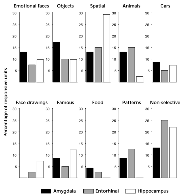
Fig. 5. Distribution of selective neurons for each category. The percentage of neurons selective for each category of stimuli and the percentage of nonselective neurons are shown for each location (black, amygdala; gray, entorhinal cortex; white, hippocampus). The percentages are based on the total number of responsive neurons in each location. Data from the right and left hemisphere have been pooled. A neuron was considered to be visually selective if the activity during stimulus presentation for a given category was significantly different from the baseline and from the neuronal response to other categories. If the response was different from baseline but not among the different categories, the neuron was defined as nonselective.
