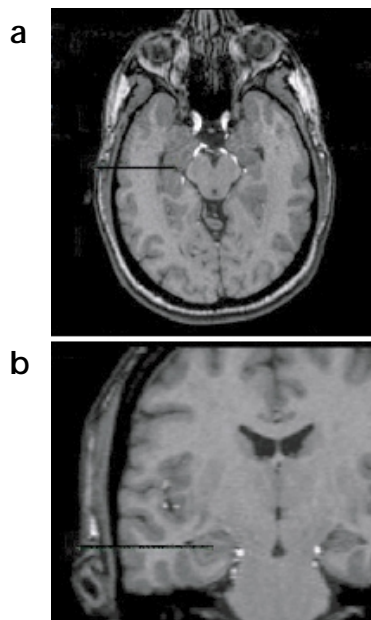
Fig. 1. Electrode placement. The trajectory of an electrode placed in the hippocampus is depicted in axial ( a ) and coronal (detail, b ) structural MR images (1.5 Tesla scanner). Post-operative CT and MRI were used to confirm the location of the electrode. The CT was co-registered with MRI structural information for anatomic verification. The distal end of the electrode included platinum-iridium microwires from which single neurons were recorded. The microwires extended about 4 mm from the tip, lying on a cone with an opening angle of less than 45 degrees.
